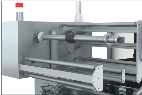
Directly Servo-driven reel shaft (T ver)
