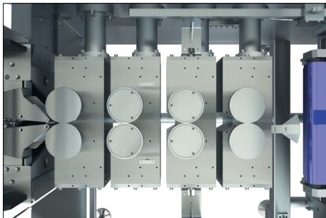
Longitudinal sealing station (T version)
